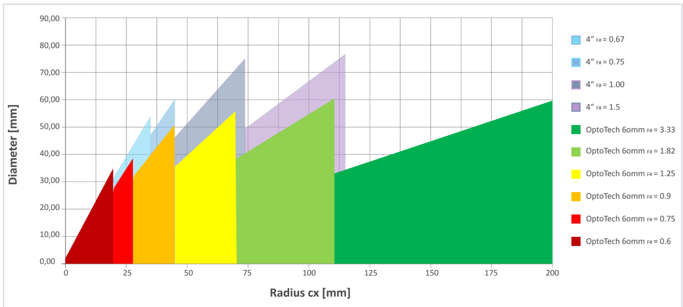
Comparison: Measuring range OptoTech 60mm reference spheres vs. measuring range 4" reference spheres
